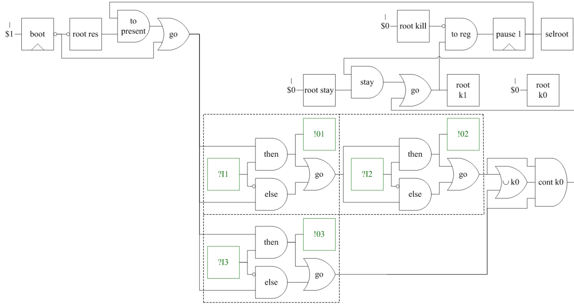
Figure 4.7: Circuit du programme Esterel 4.3 (ReconvergentBranches)
