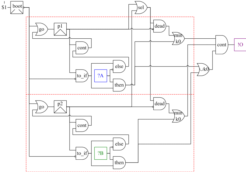
Figure 2.2: Le circuit AB_O
