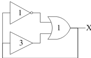
Figure 2.4: Le circuit “Hamlet”
